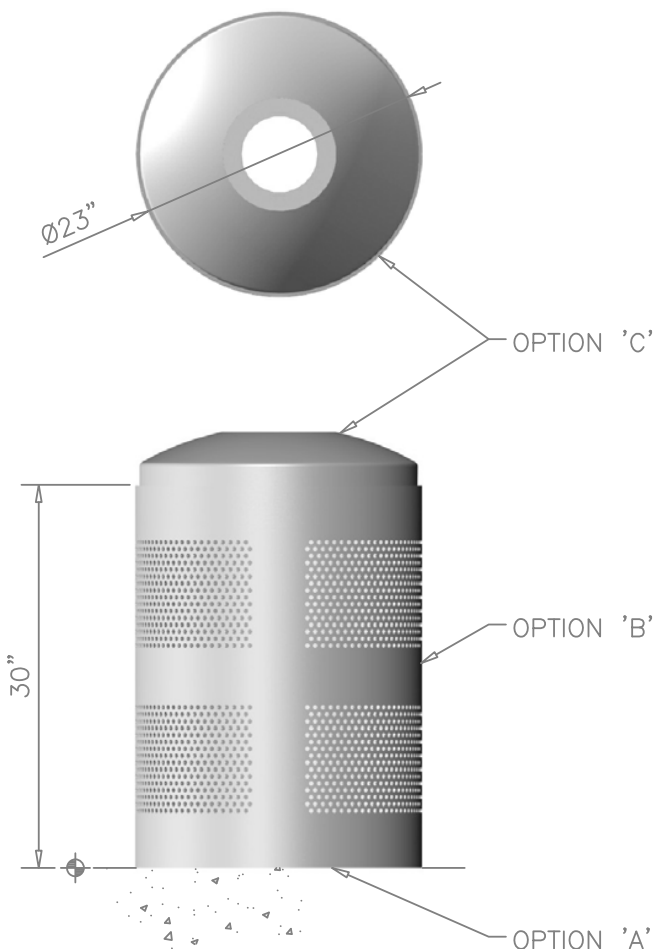
LITTER RECEPTACLE BELLE ISLE SERIES
